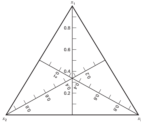
■ FIGURE 11.40 Trilinear coordinate system
