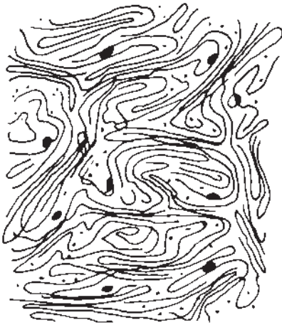
10.2 Pore model of dye diffusion.
