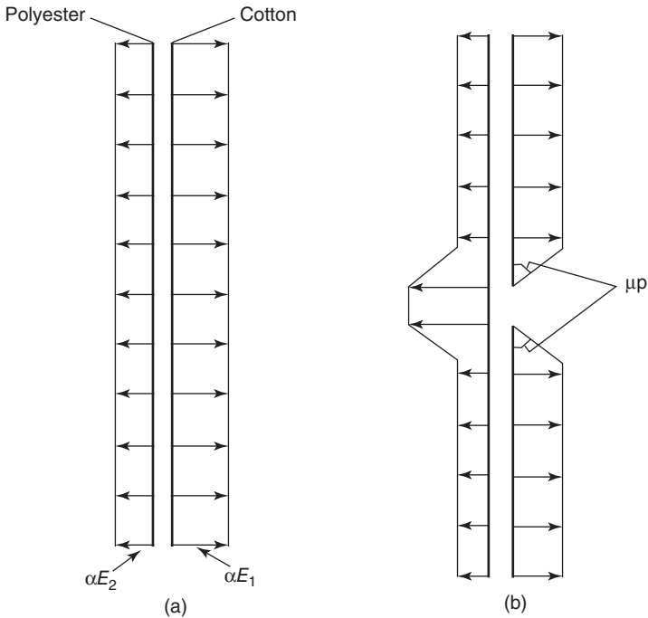
8.18 Stress transfer between fibres. 13 (a) 2% elongation, (b) 10% elongation. ( \alpha ) local strain; (E) tensile modulus; ( \mu ) coefficient of friction; (p) local pressure.
