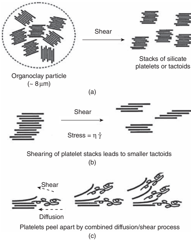
13.18 Mechanism of exfoliation of clays: (a) organoclay particle break up; (b) clay tactoid break up; (c) platelet exfoliation.
