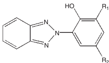
Benzotriazoles
