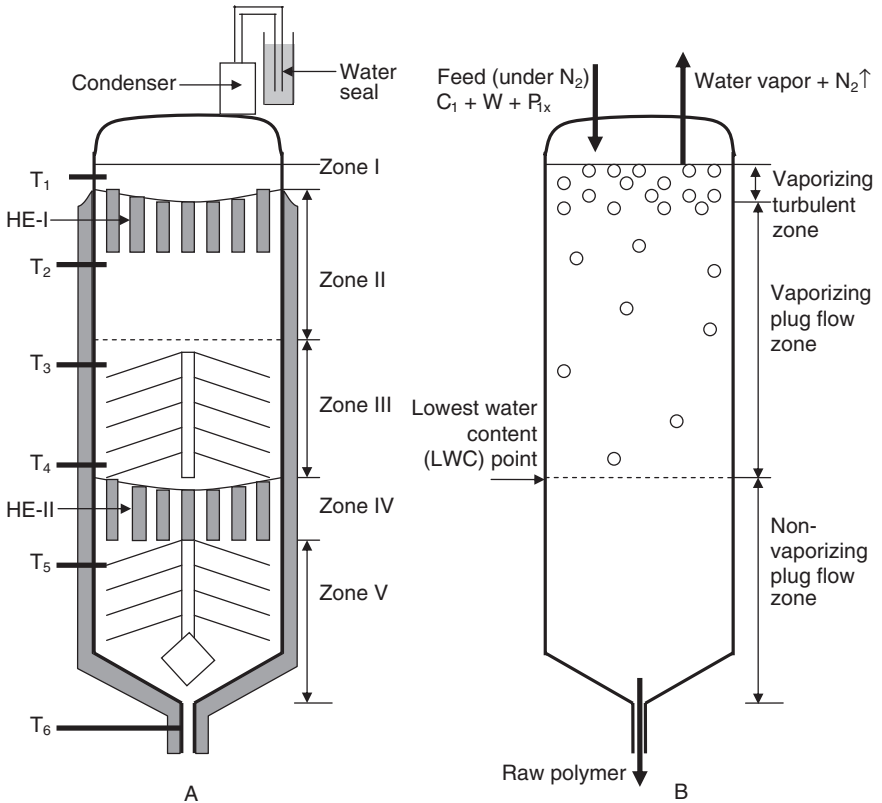
4.4 VK tube reactor: (A) Schematic diagram of industrial VK tube reactor depicting the various heating zones (zone I – zone V), heat exchangers (HE-I and HE-II) and temperature measuring points ( T_1 to T_6 ); (B) VK tube reactor model consisting of three main zones: Vaporizing turbulent (top) zone, vaporizing plug flow zone and non-vaporizing plug flow zone.
