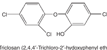
12.1 Molecular structures of two antimicrobial agents.
